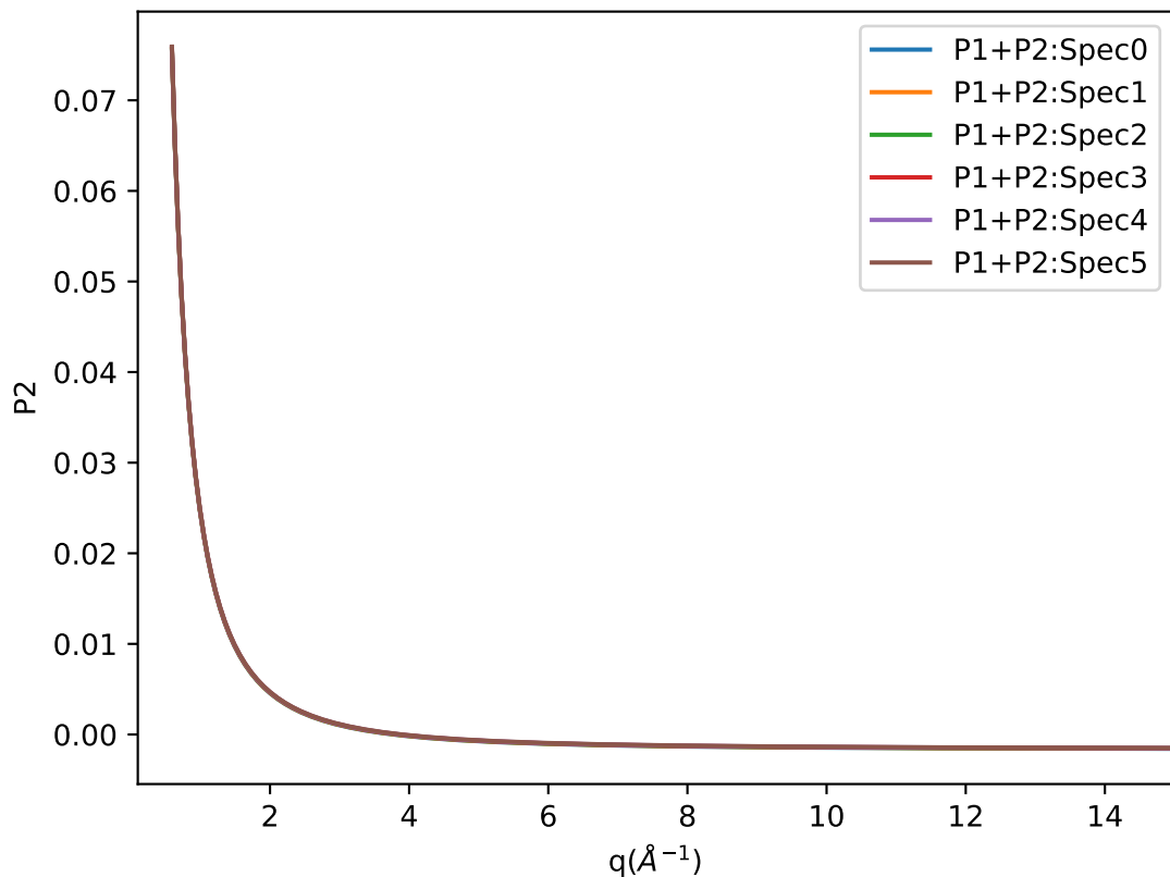
Full Placzek correction factor (P1+P2)
