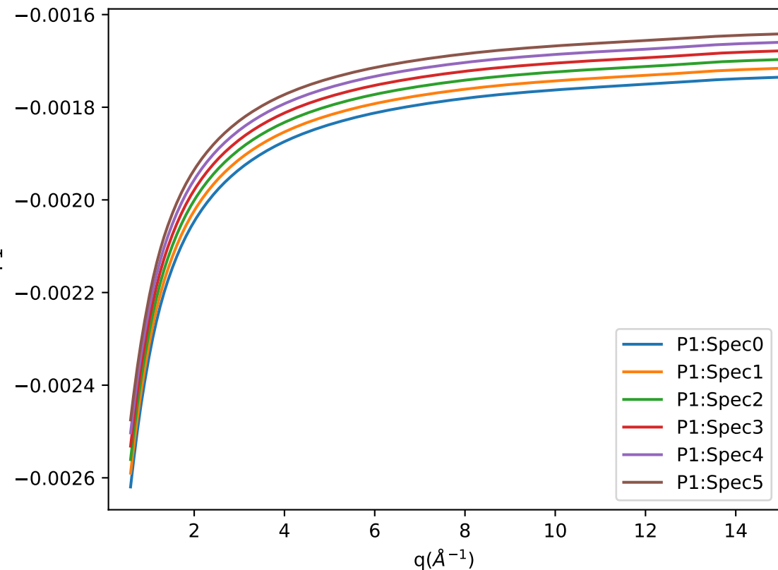
First Order Placzek correction factor
