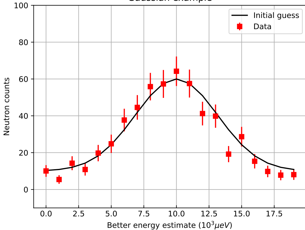
Gaussian example
